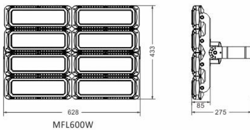
MFL600W
