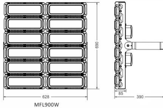
MFL900W
