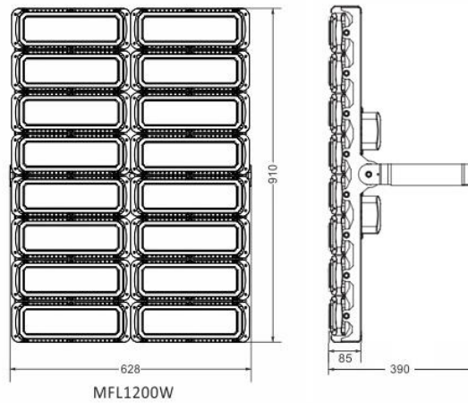
MFL1200W
