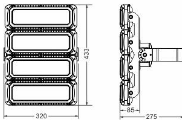
MFL300W
