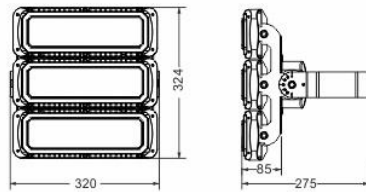
MFL230W
