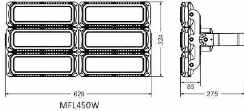
MFL450W
